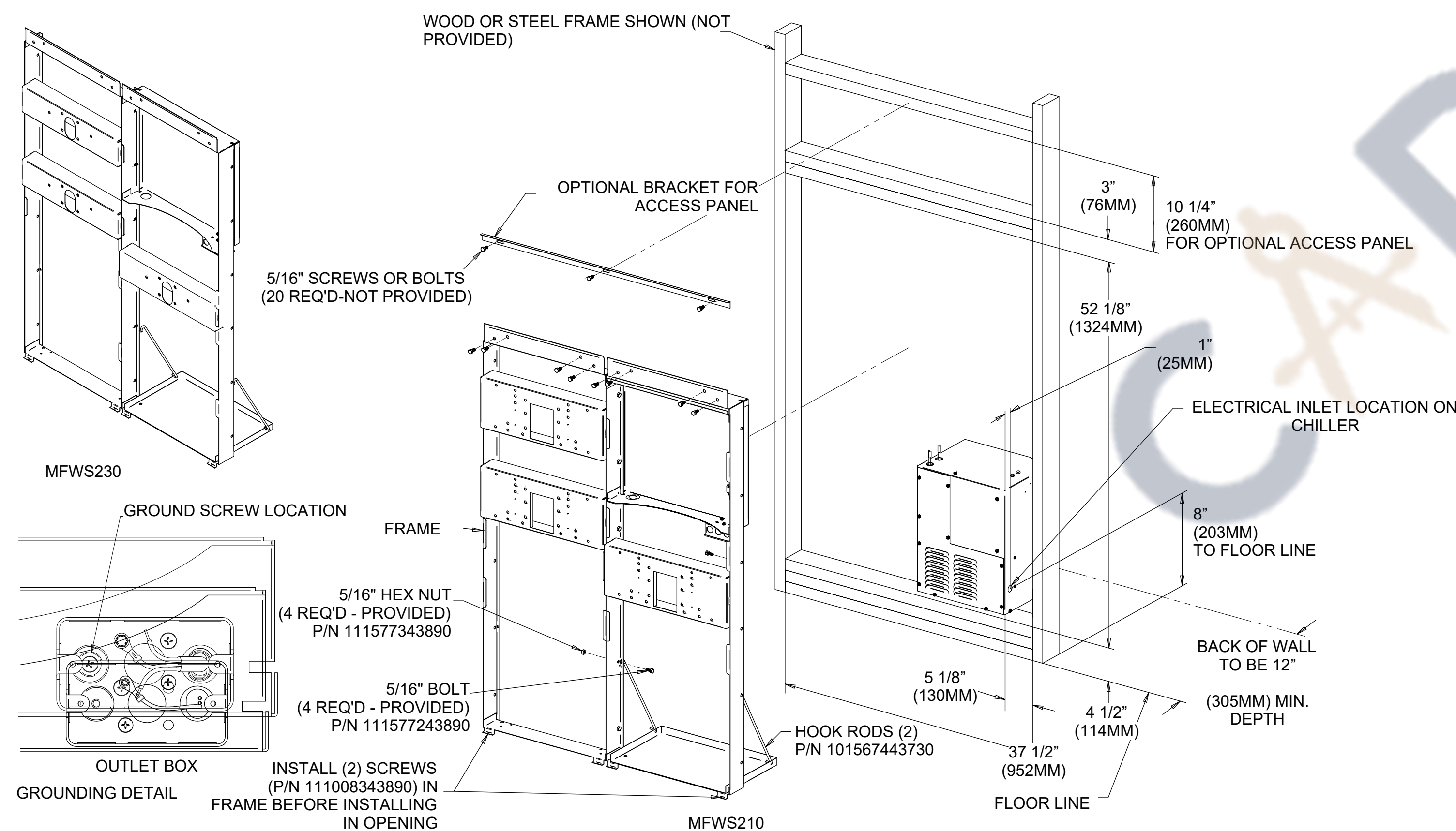
④ EWC MOUNTING FRAME INSTRUCTIONS 1 1/2" = 1'-0"
