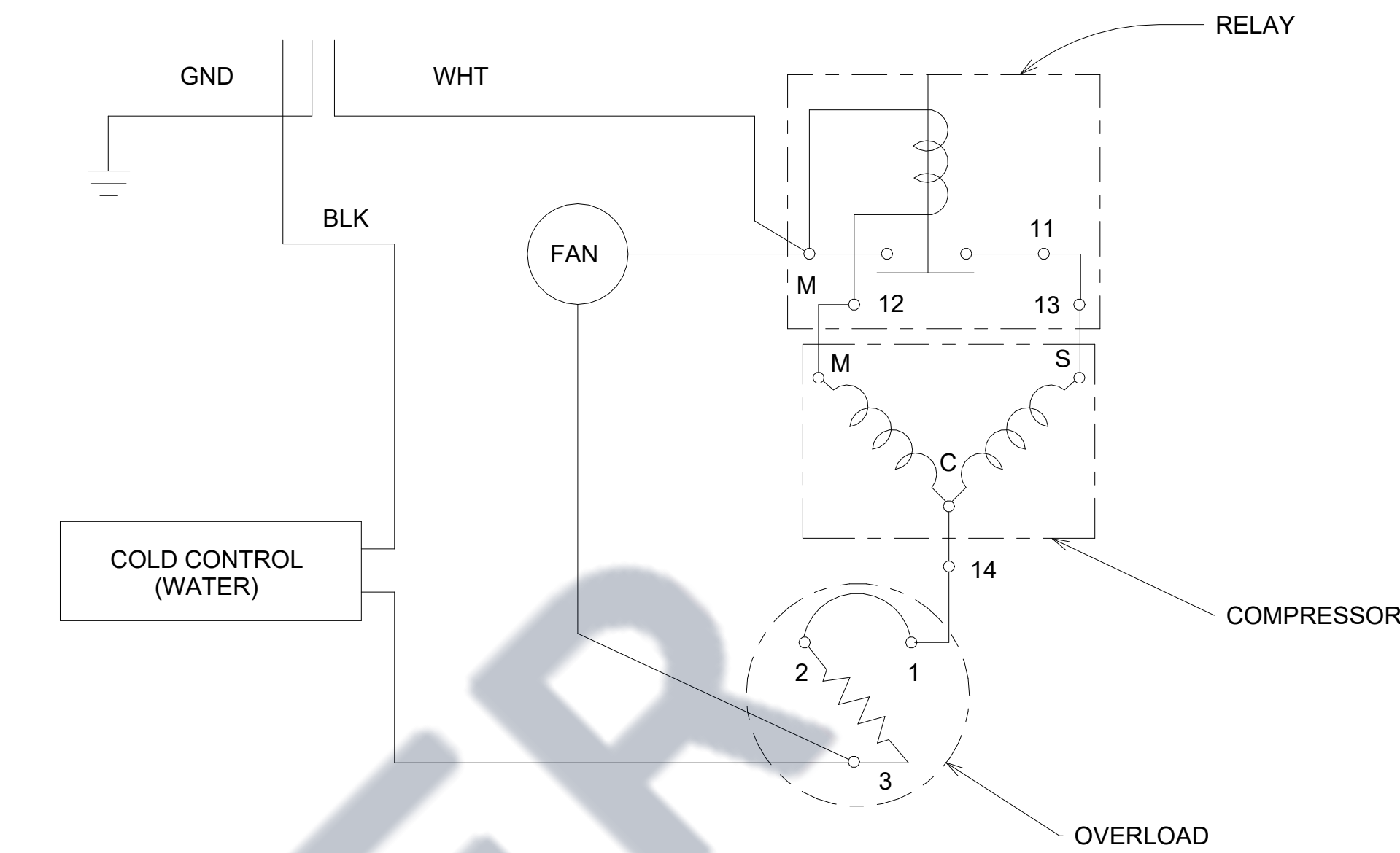
⑤ WIRING DIAGRAM 1 1/2" = 1'-0"
