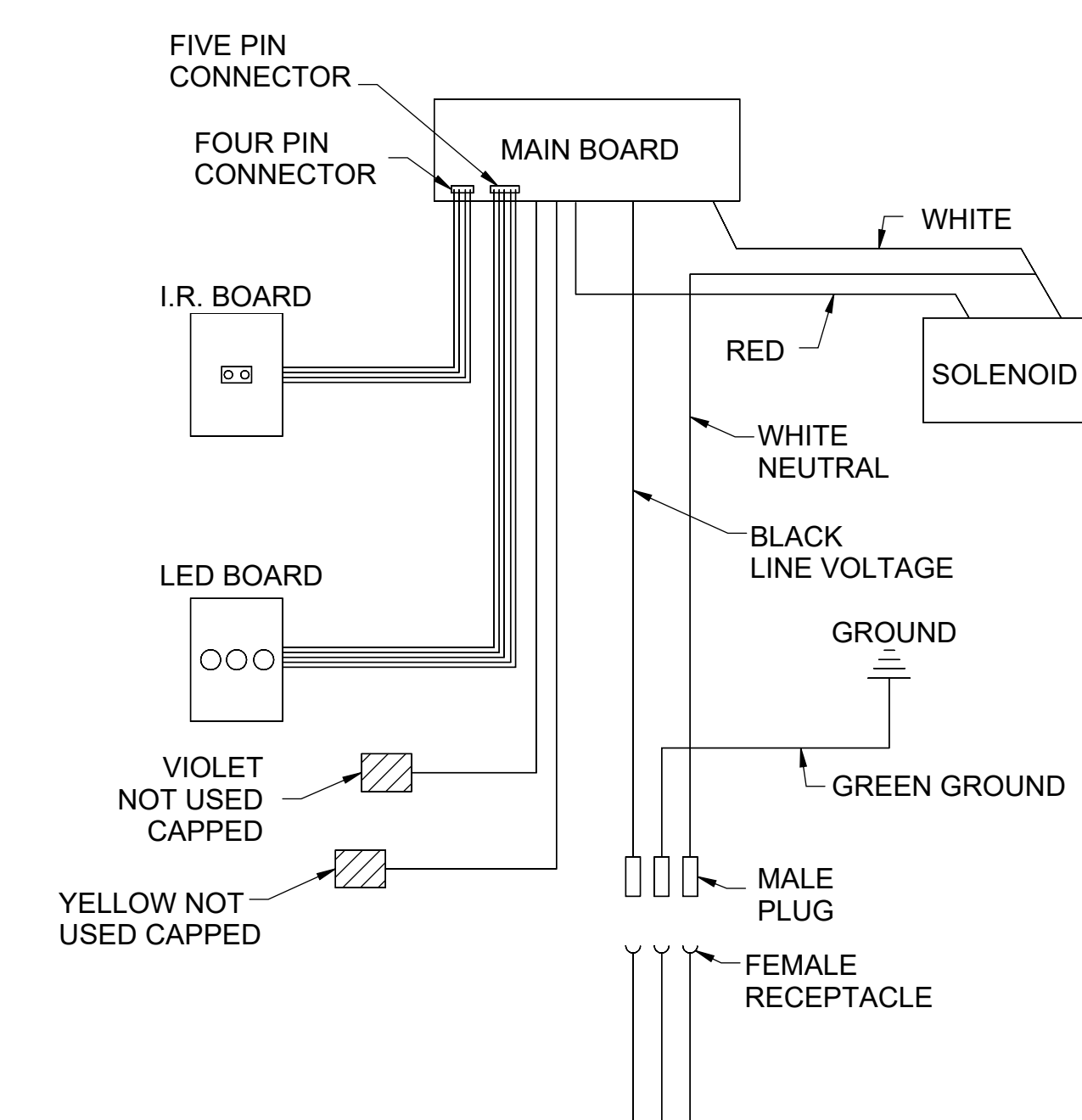
③ EWC Electrical Diagram 1 1/2" = 1'-0"
