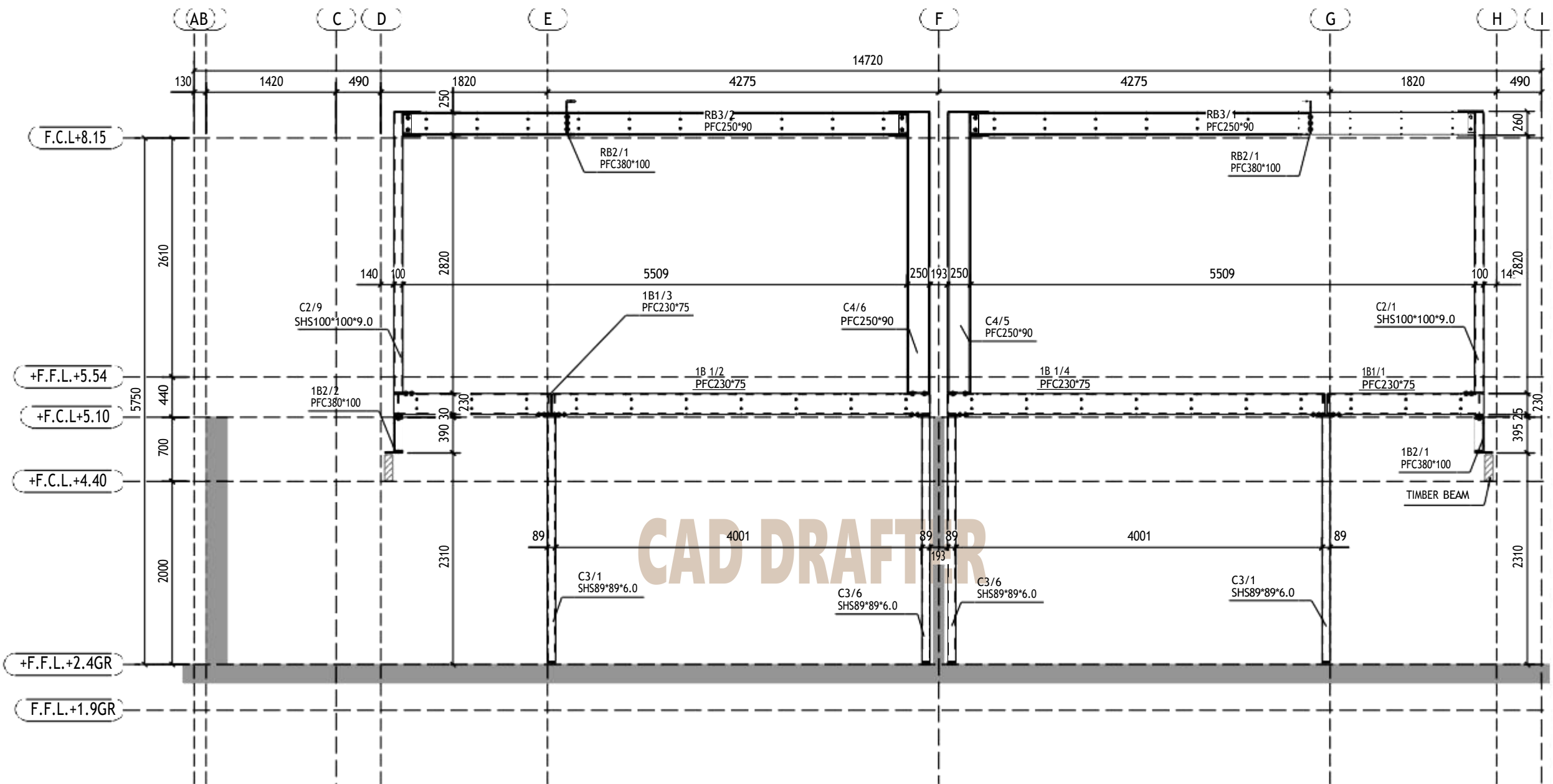
F - F BEAM LAYOUT PLAN
